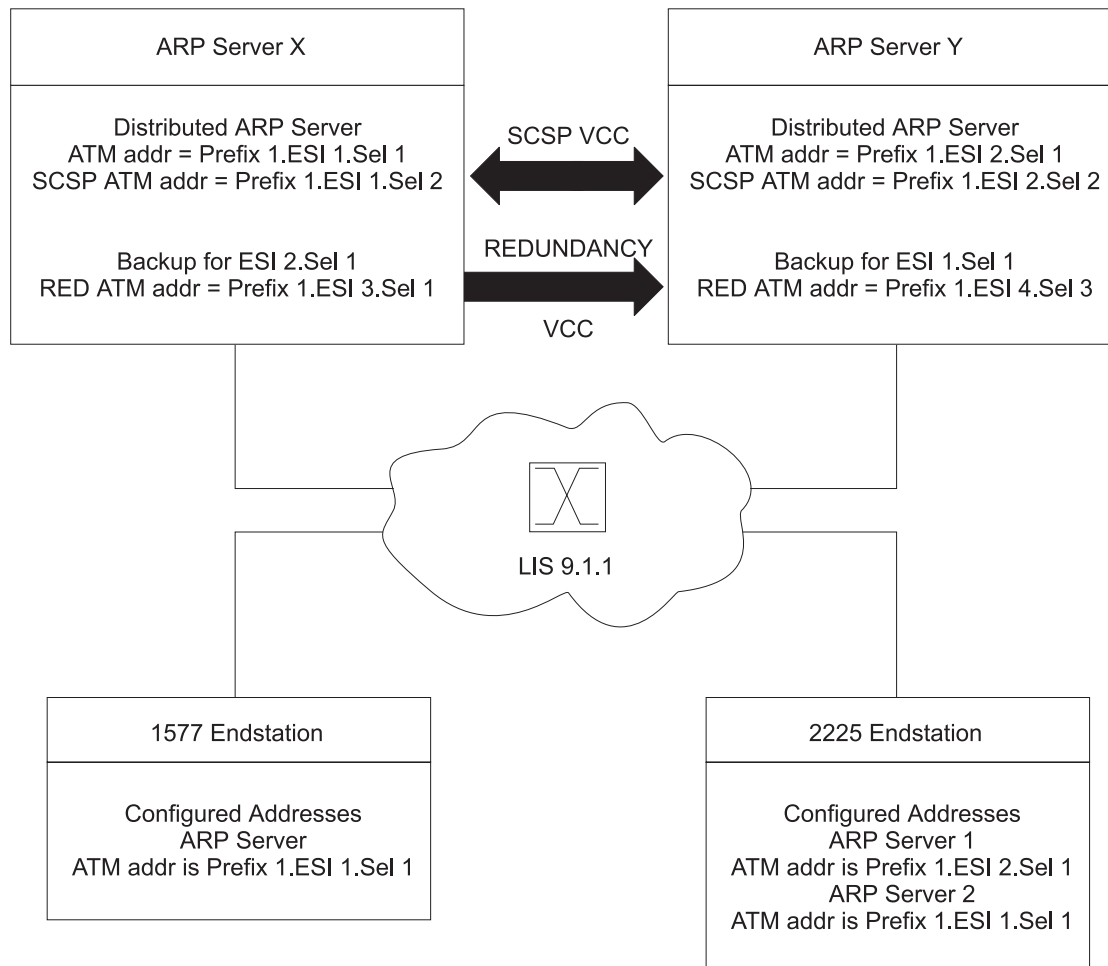
Figure 37. ARP Server Configuration with RFC 1577 and 2225 Clients
