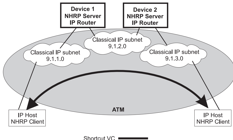
Figure 45. NHRP in a Classic IP Environment
