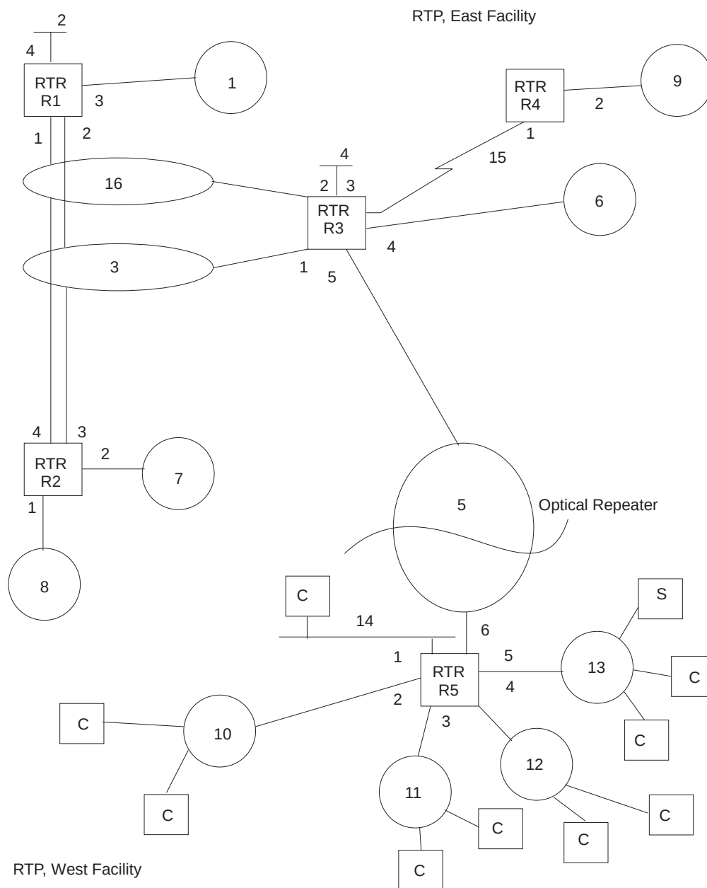
Figure 32. Sample IPX Network
