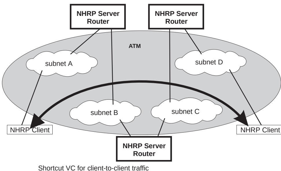
Figure 44. Next Hop Resolution Protocol (NHRP) Overview
