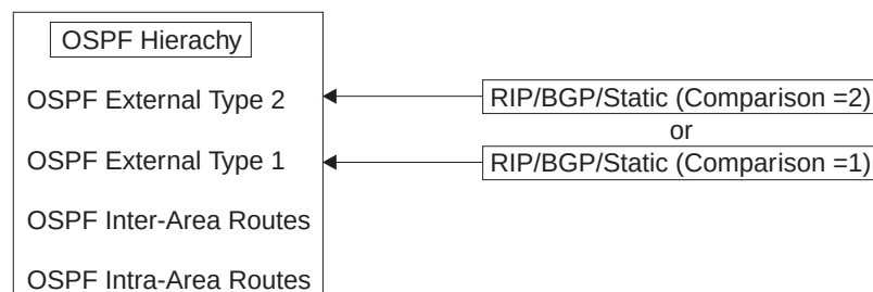
Figure 31. OSPF Routing Hierarchy
