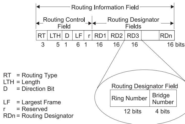
Figure 11. 802.5 Routing Information Field
