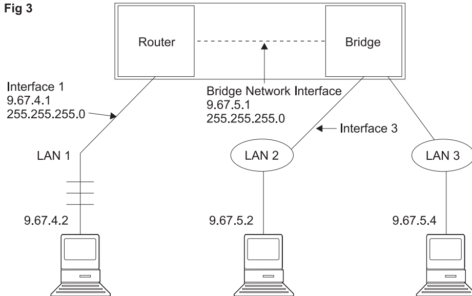
Figure 28. Routing to a Bridged Network-Alternative 3
