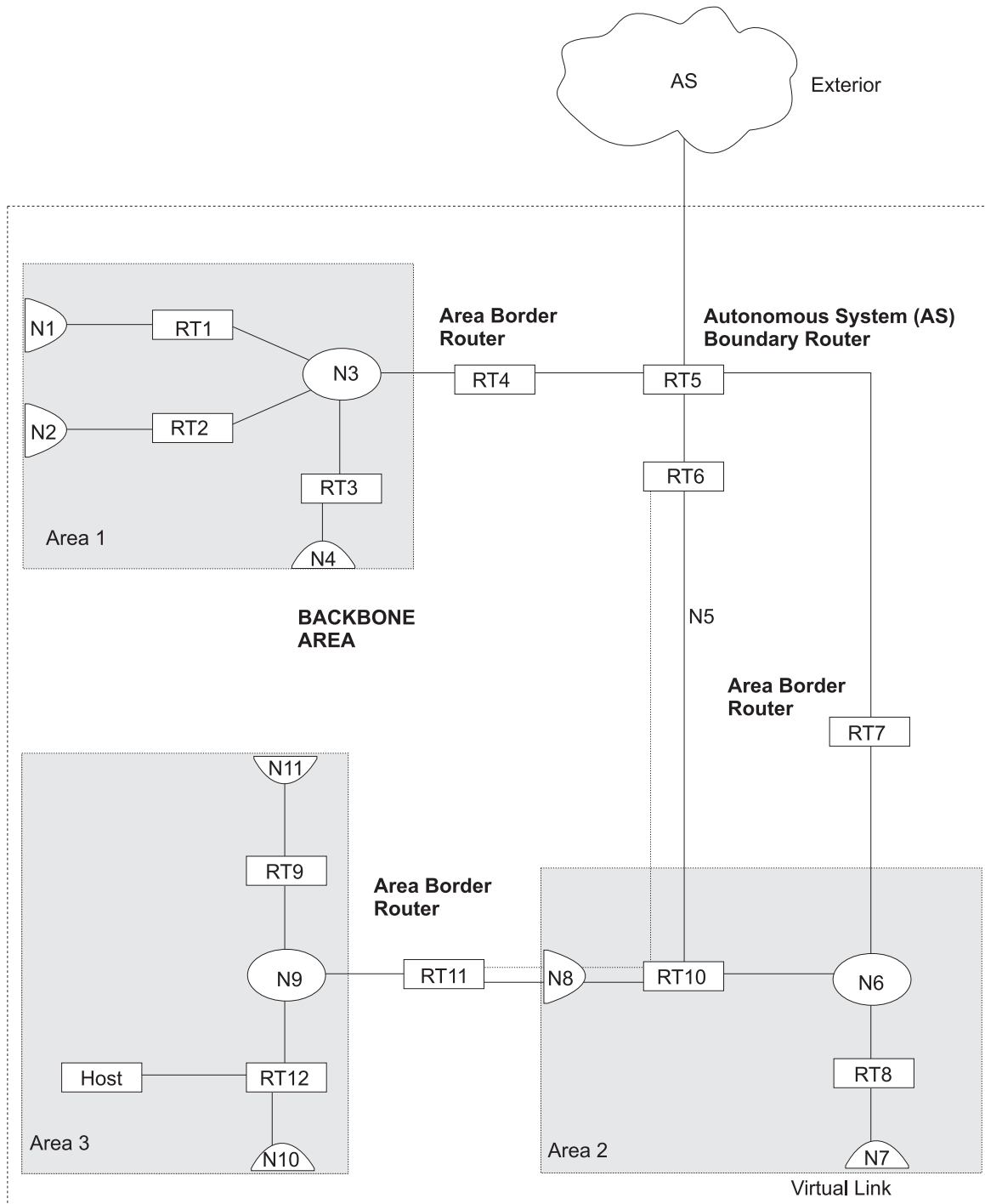
Figure 30. OSPF Areas
