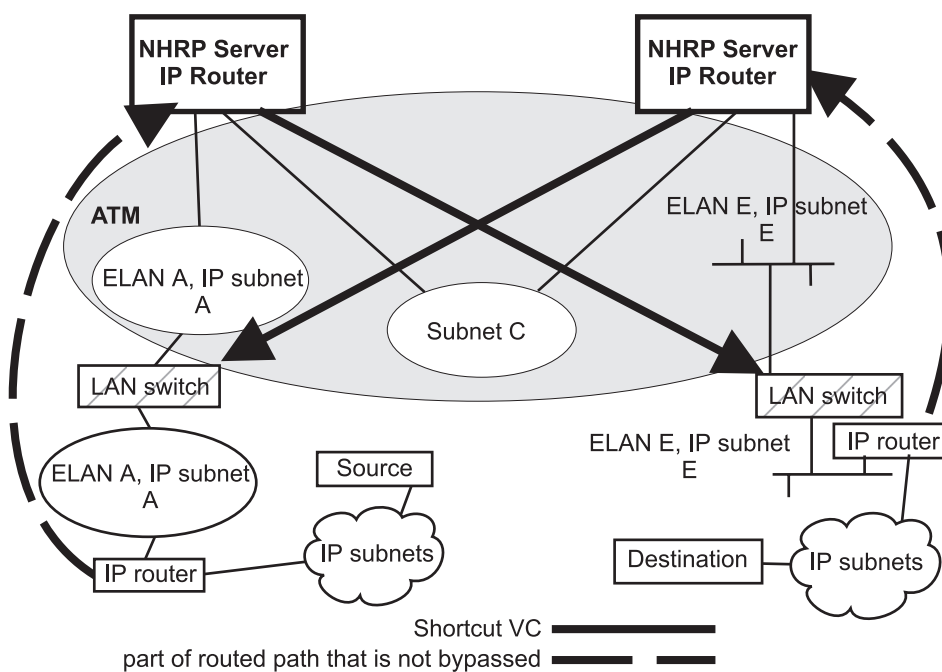
Figure 50. NHRP to an Egress Router
